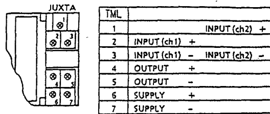
Fig.9 Wiring Diagram
